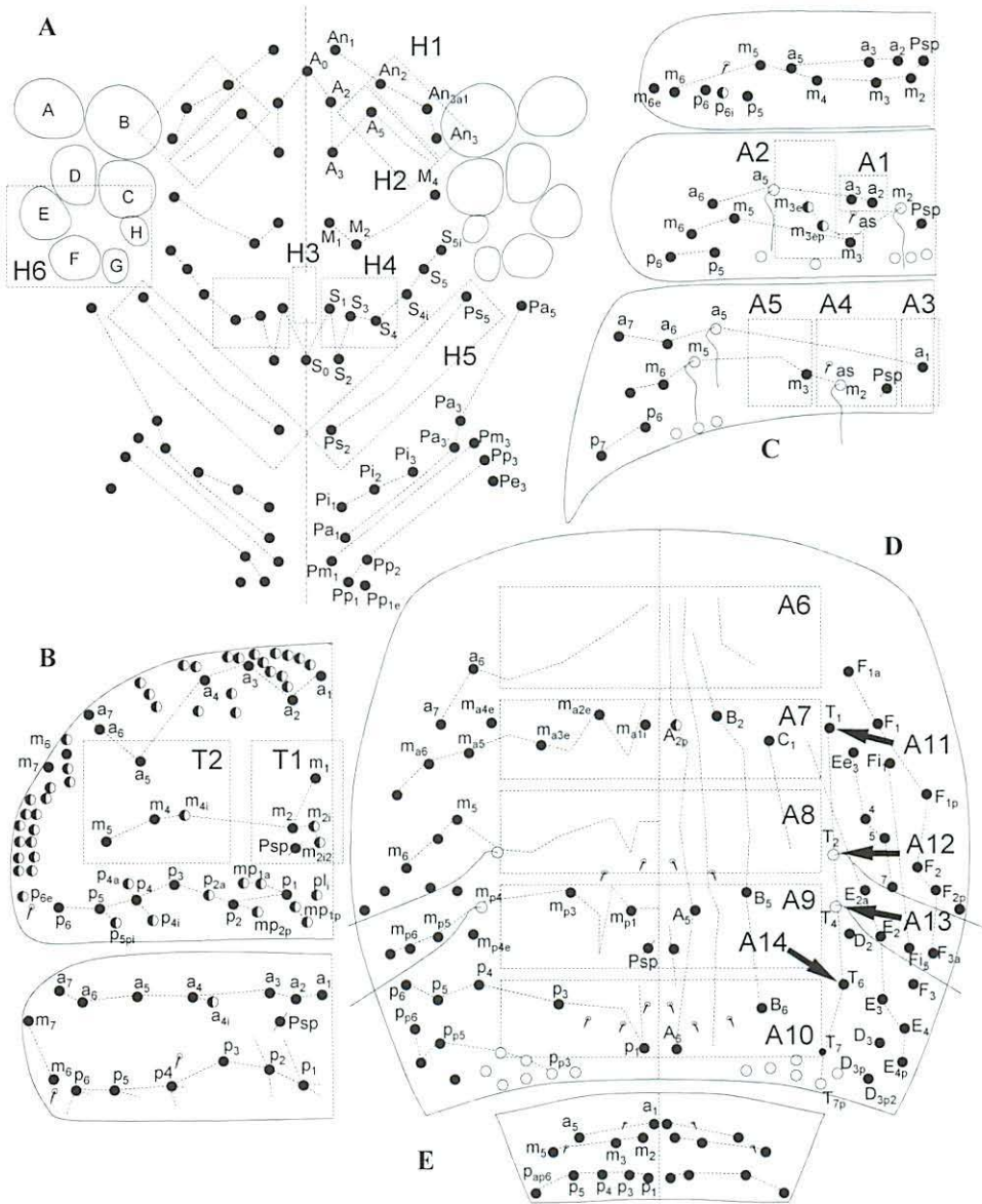
Fig. 2 E. nivalis : chaetotaxy. A head; B thoracic tergites II and III; C abdominal tergites I – III; D abdominal tergite IV; E abdominal tergite V.
