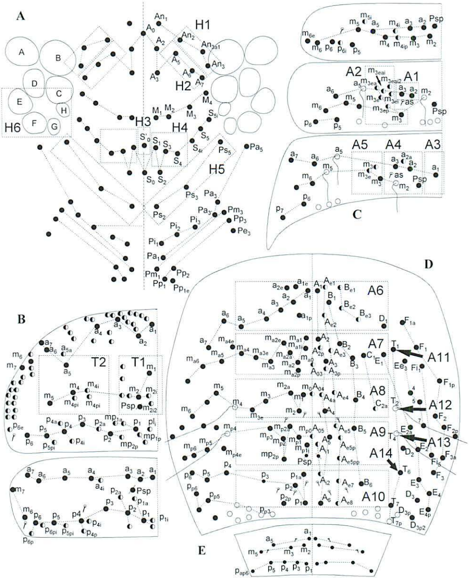
Fig. 1 Generalised chaetotaxy for Entomobrya after SZEPTYCKI (1979), SOTO-ADAMES (personal communication), MARI-MUTT (1978). A head; B thoracic tergites II and III; C abdominal tergites I – III; D abdominal tergite IV; E abdominal tergite V. Signature of insertion points of setae: full circle: primary setae; half shaded circle: secondary setae; open circle: additional setae; circle with diagonal line: pseudoporus; circle with long fine line: trichobothrium.
