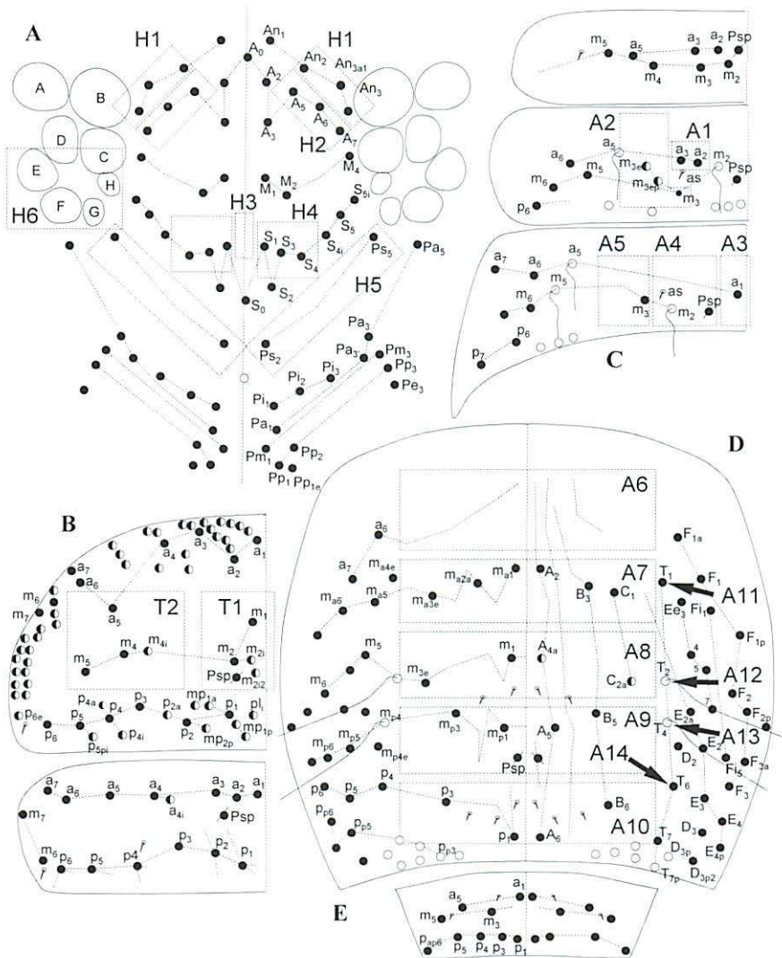
Fig. 5 E. leonensis n. sp.: chaetotaxy. A head; B thoracic tergites II and III; C abdominal tergites I – III; D abdominal tergite IV; E abdominal tergite V.
